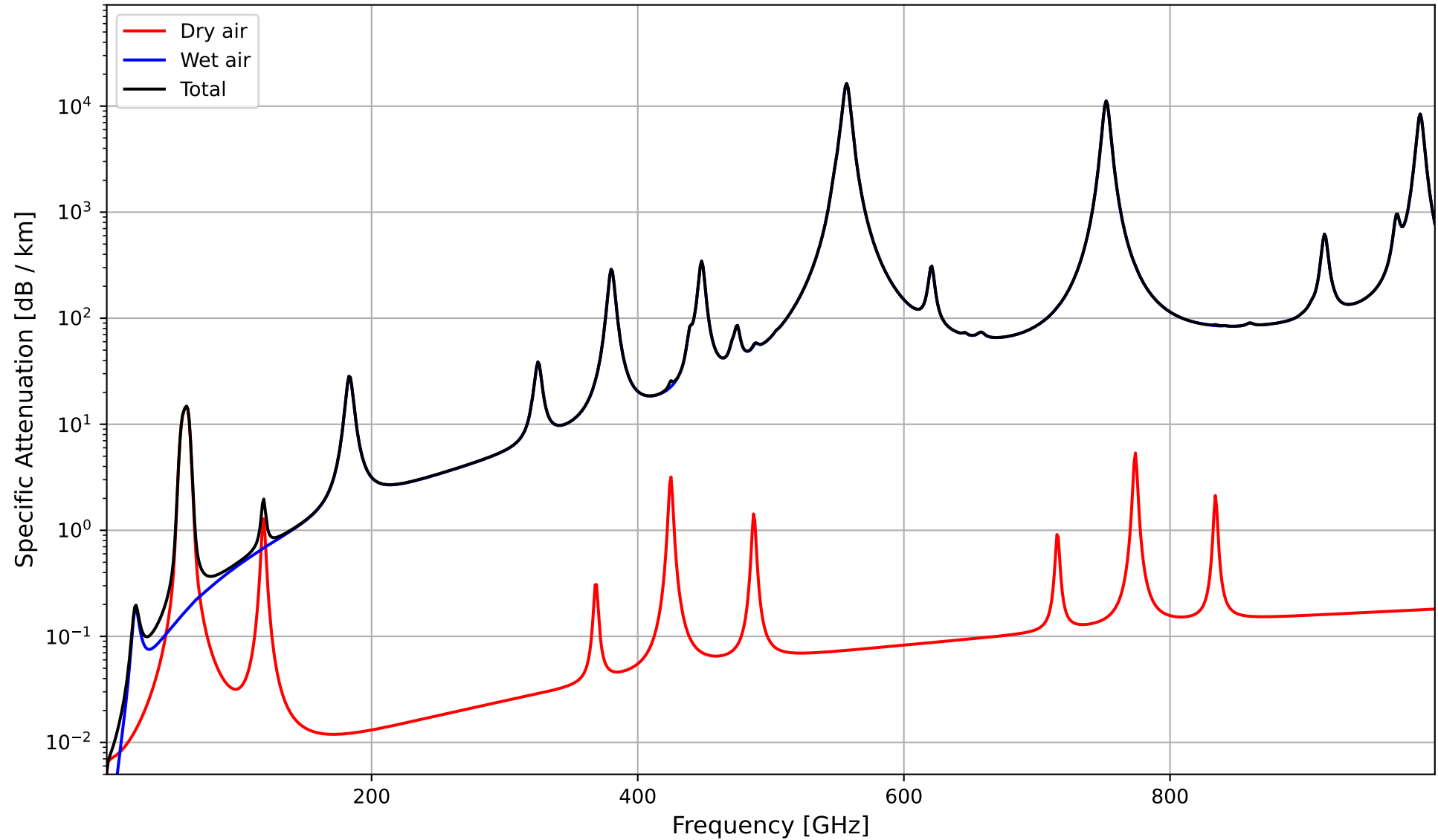
Specific attenuation for standard conditions, according to ITU-R P.676 (10), annex 1
