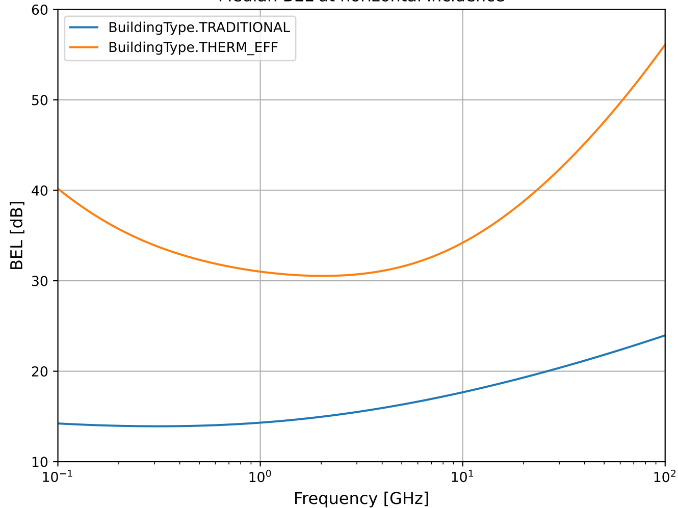
Median BEL at horizontal incidence
