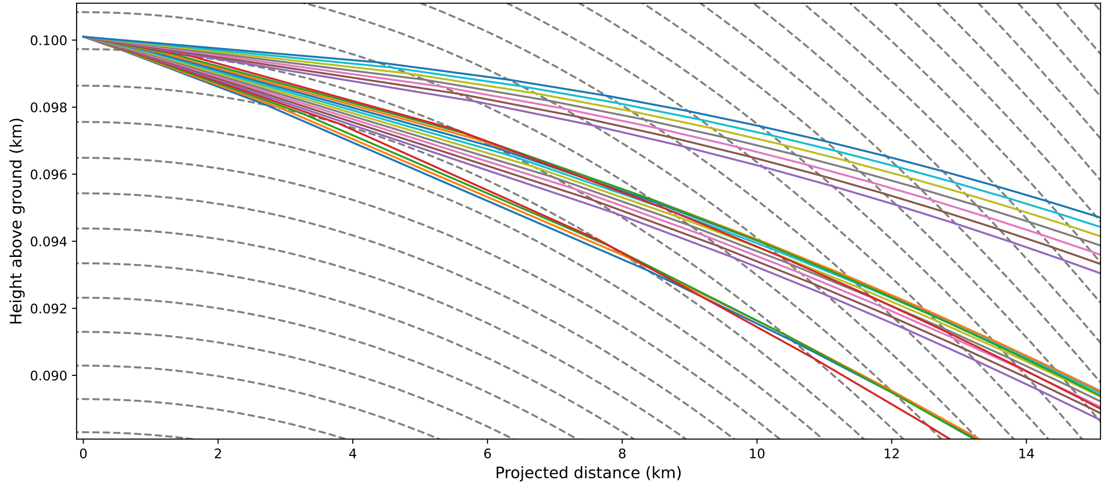
Path propagation through layered atmosphere
