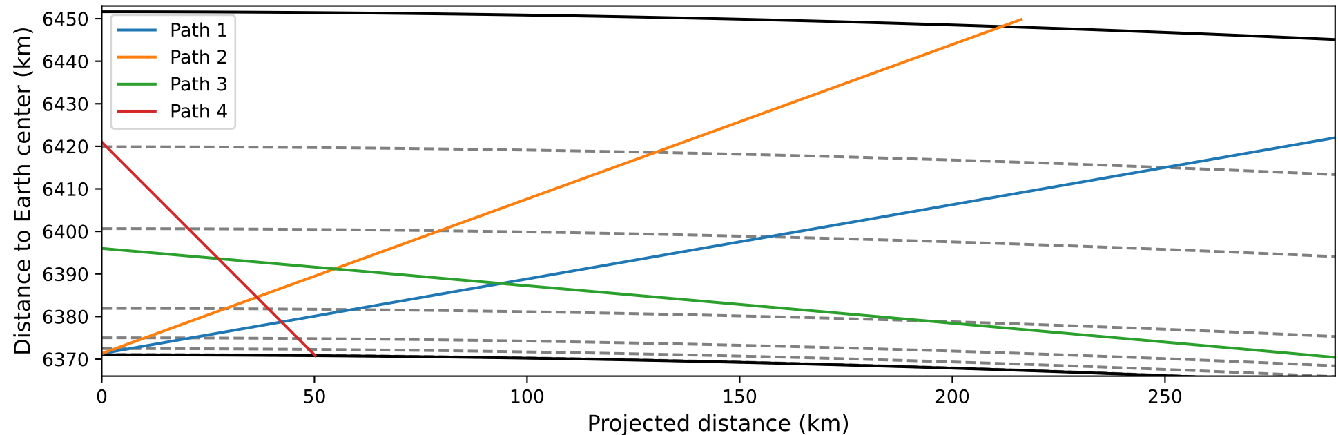
Path propagation through layered atmosphere
