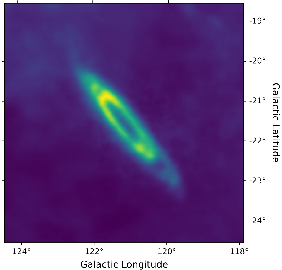
EBHIS 21-cm HI line
