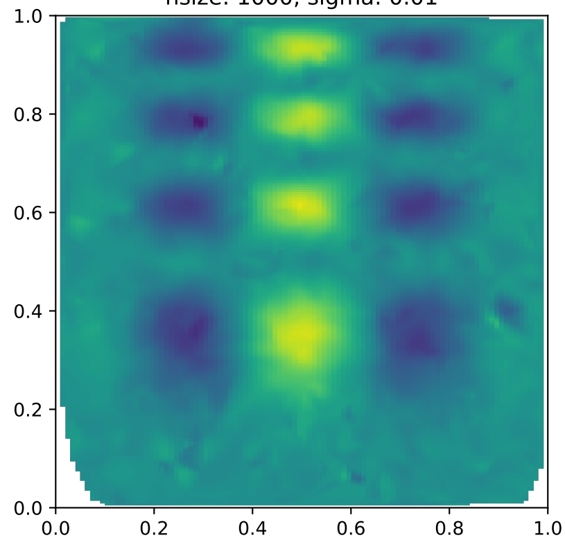
nsize: 1000, sigma: 0.01
