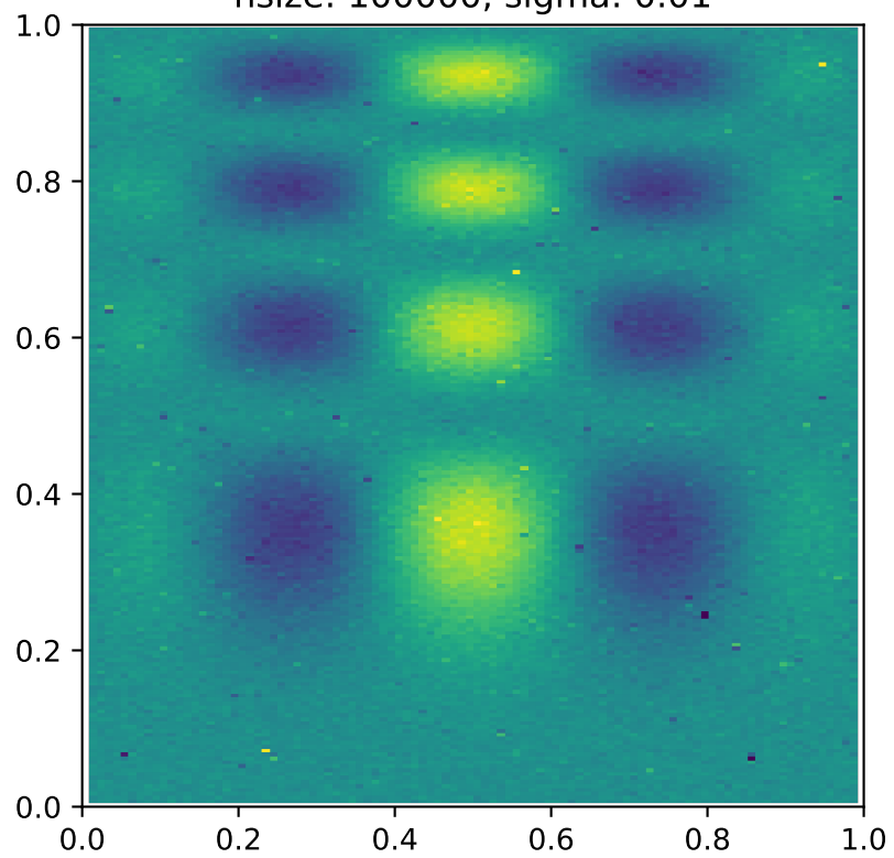
nsize: 100000, sigma: 0.01
