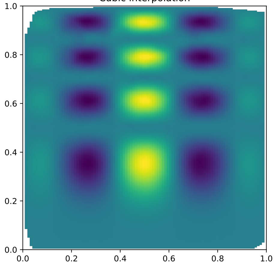
Cubic interpolation
