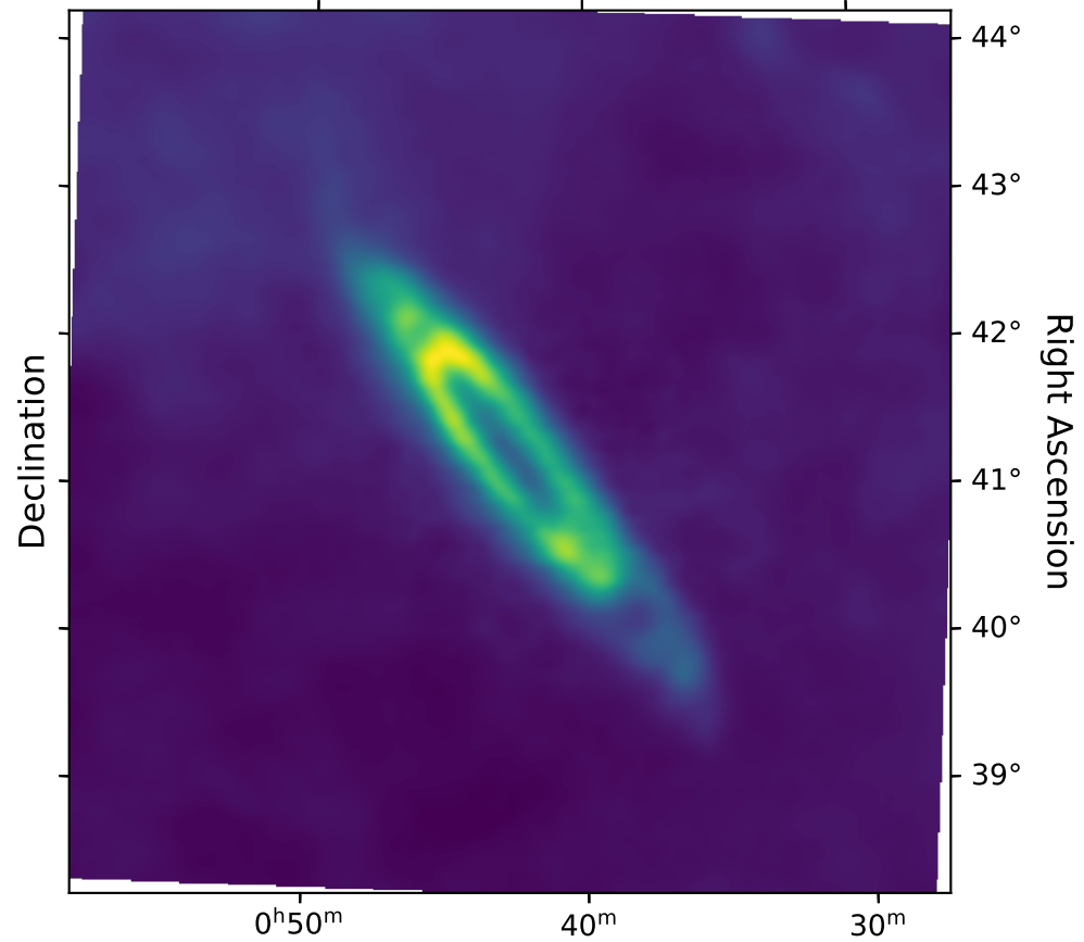
EBHIS 21-cm HI line
