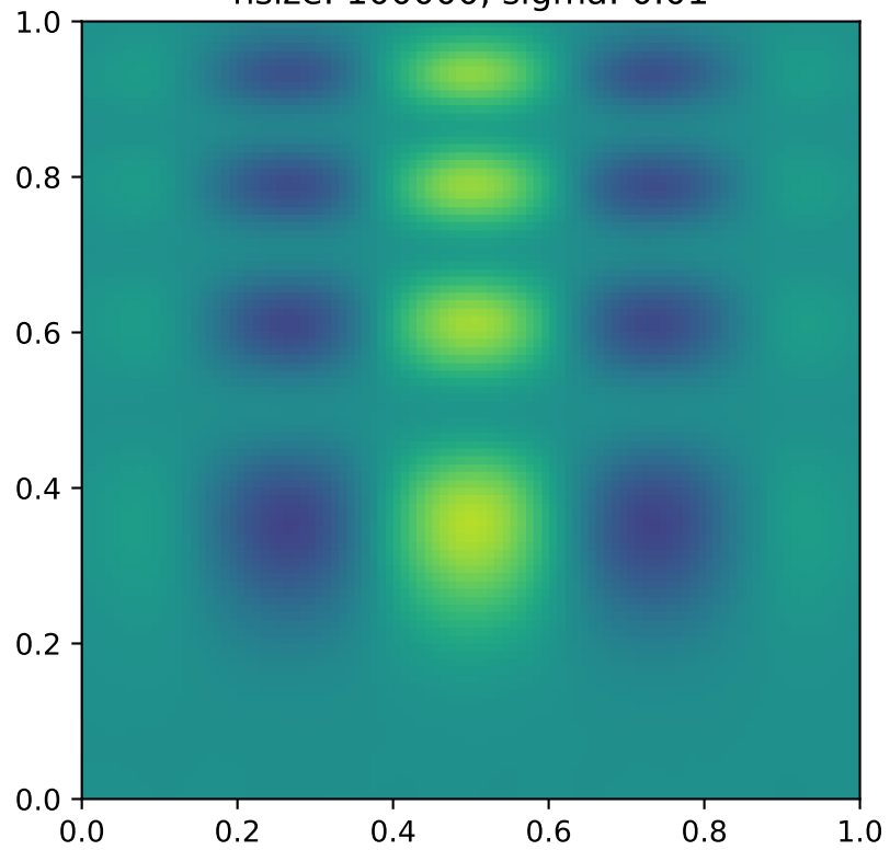
nsize: 100000, sigma: 0.01
