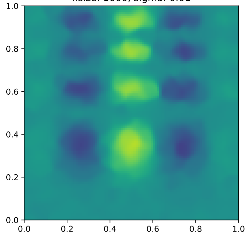
nsize: 1000, sigma: 0.01
